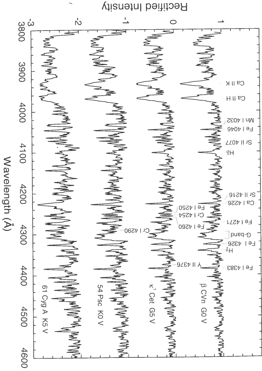
Figure 7.1 A temperature sequence for main-sequence stars from G- to mid-K types. Features useful in the temperature classification of these stars are marked. These spectra have been rectified and offset vertically by 0.7 continuum units. Unless otherwise stated, all spectra in this chapter were obtained at the Dark Sky Observatory.
